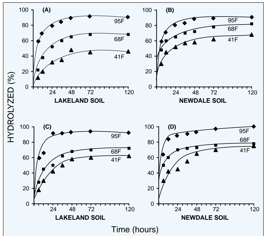
Figure 2. Temperature effect on hydrolysis of water-soluble sodium pyrophosphate and sodium tripolyphosphate. A and B = 200ppm pyrophosphate; C and D = 200ppm tripolyphosphate.
