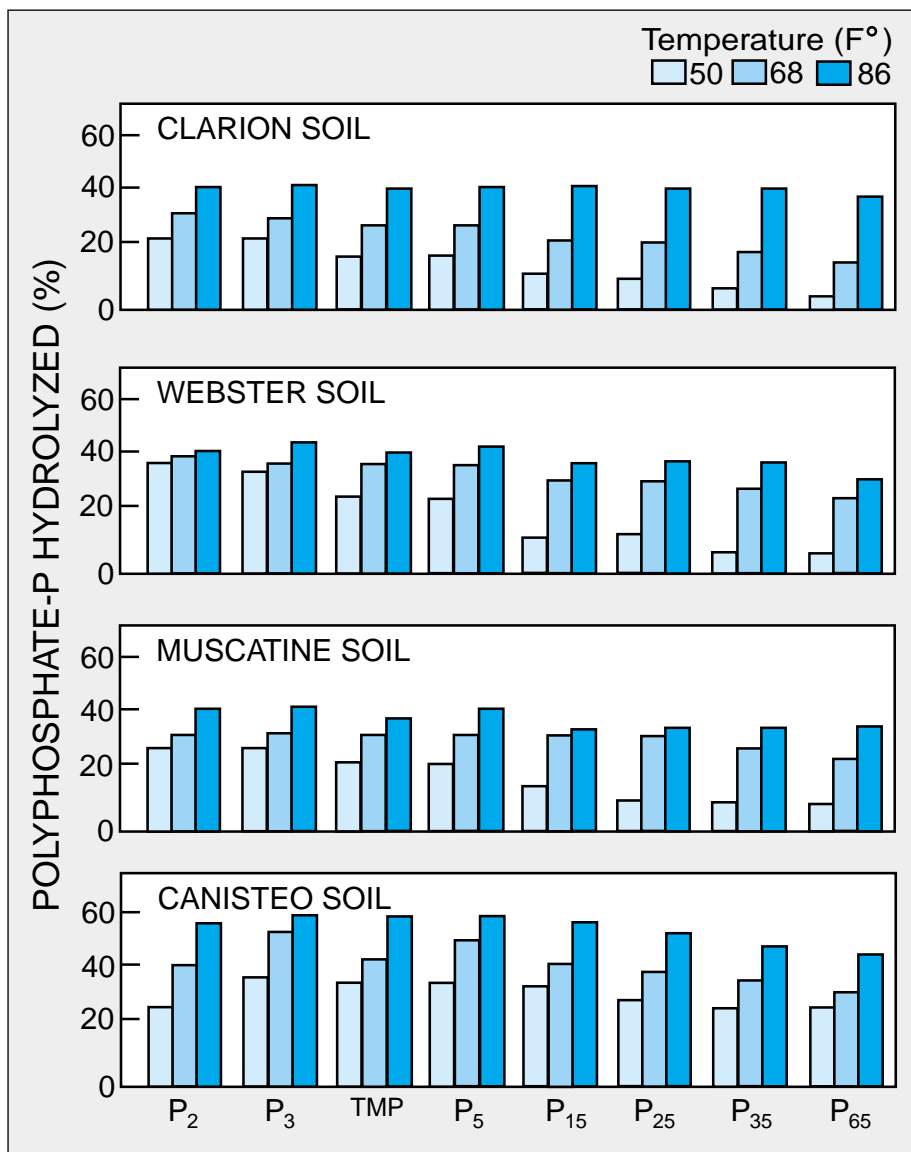
Figure 1. Effect of temperature on hydrolysis of polyphosphates in soils incubated for seven days.
